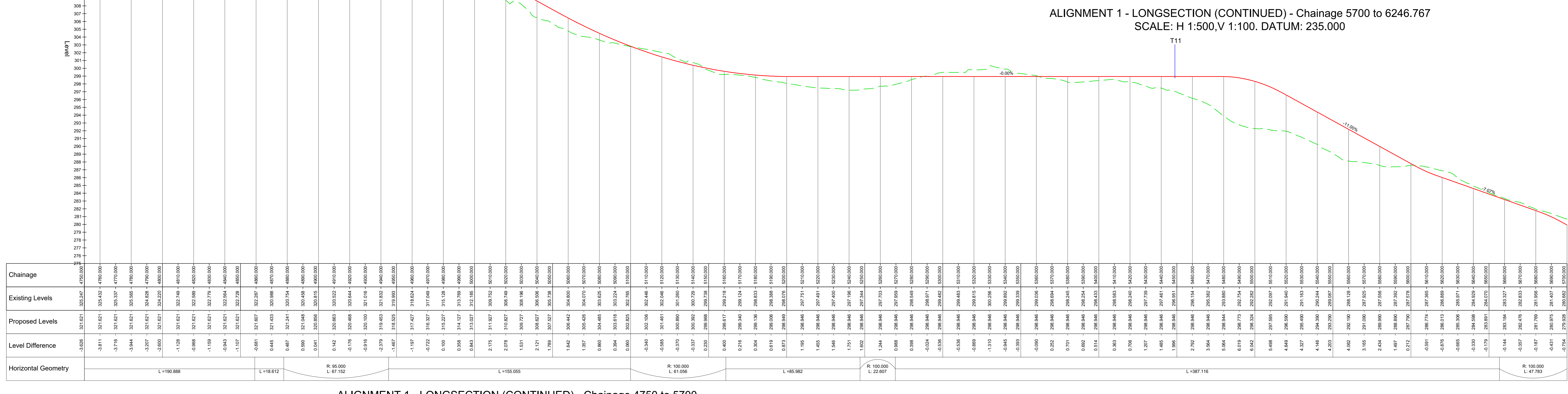
ALIGNMENT 1 - LONGSECTION (CONTINUED) - Chainage 5700 to 6246.767 SCALE: H 1:500,V 1:100. DATUM: 235.000
